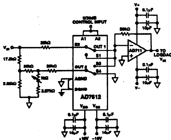
Figure 3. Fixed Attenuator
